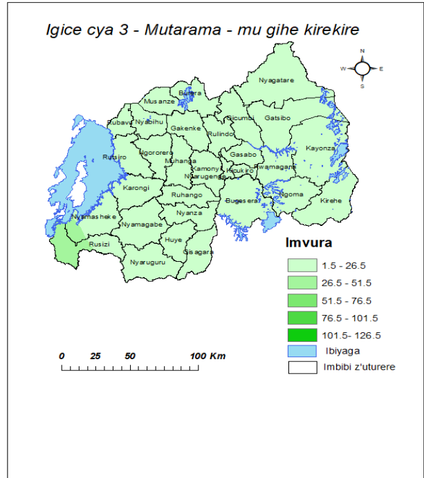
Ishusho 2:Imvura isanzwe igwa mu gice cya gatatu cy'ukwezi kwa Mutarama
