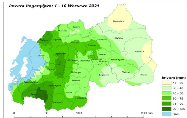
Ikarita ya 6: Iteganyagihe ry'imvura mu gice cya mbere cya Werurwe 2021.
