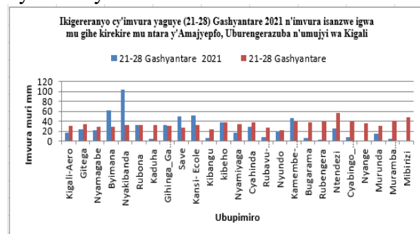
Ishusho 1 : ikigereranyo cy'imvura mu Mujyi wa Kigali, Intara y'Amajyepfo n'iy'Iburengerazuba
