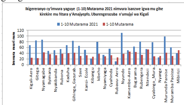
Ishusho 1: ikigereranyo cy'imvura mu mujyi wa Kigali, intara y'Amajepfo niy'Iburengerazuba
