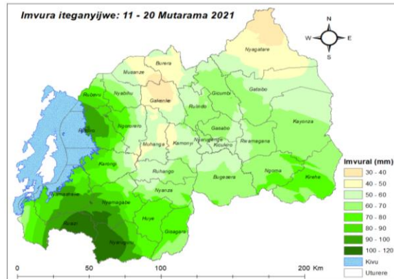
Ikarita ya 6: Iteganyagihe ry'imvura mu gice cya kabiri cya Mutarama 2021.
