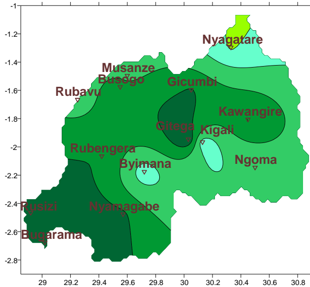
Ikarita ya1: Imvura yaguye (mm): 11-20_Ukwakira_2018
