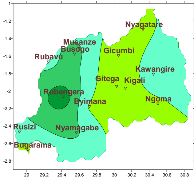
Ikarita ya1: Imvura yaguye (mm): 01-10_Ukwakira_2018
