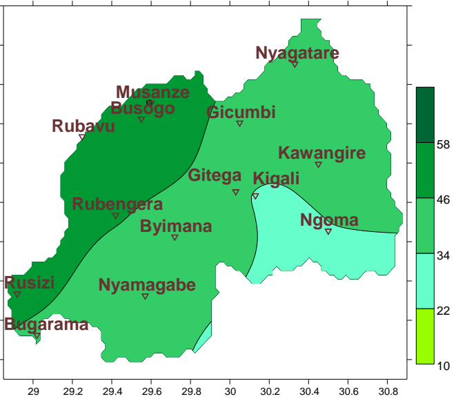
Ikarita ya2: Imvura isanzwe igwa (mm): 11-20_Ukwakira
