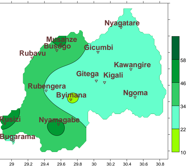
Ikarita ya2: Imvura isanzwe igwa (mm): 01-10_Ukwakira
