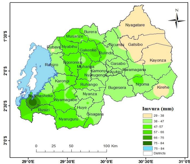
Ikarita ya 2: Imvura isanzwe igwa mu gice cya gatatu cy'ukwezi k' Ugushyingo
