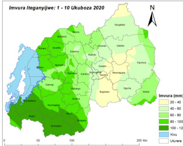
Ikarita ya 6: Iteganyagihe ry’imvura mu gice cya mbere cy’Ukuboza 2020.
