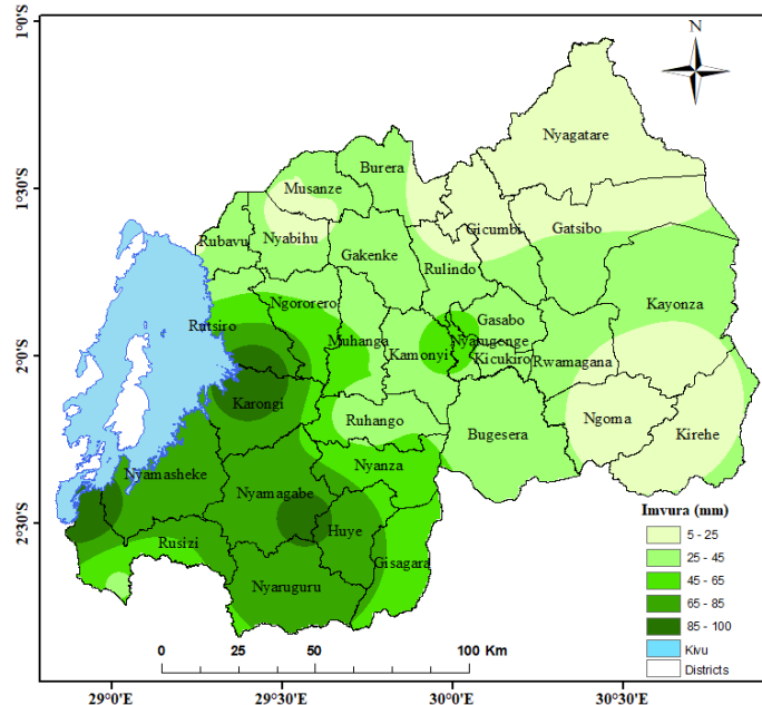
Ikarita ya 1: Ingano y'Imvura yaguye mu gice cya kabiri cy'Ugushyamba 2020
