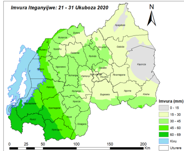
Ikarita ya 6: Iteganyagihe ry'imvura mu gice cya gatatu cy'Ukuboza 2020.
