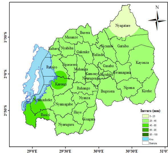
Ikarita ya 2: Imvura isanzwe igwa mu gice cya kabiri cy'ukwezi k' Ukuboza
